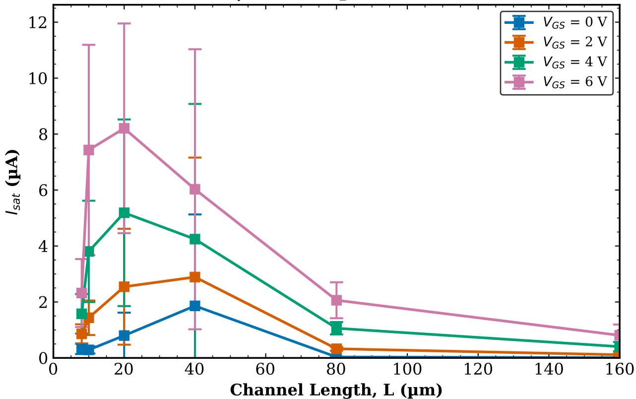
All Chips - Combined I_{sat} vs L | W = 10 \mu\text{m} (mean \pm std)
